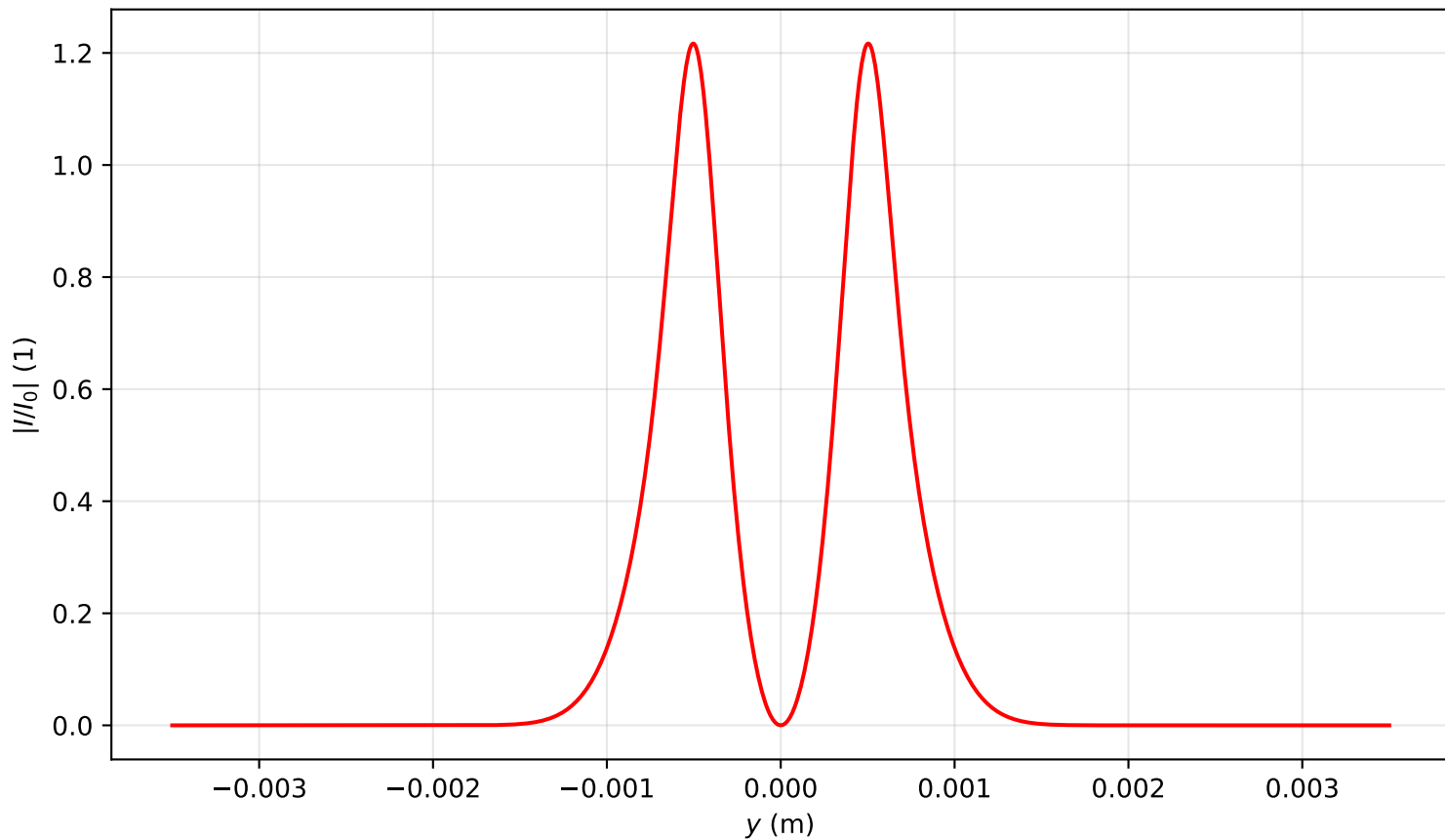
Intensity profile I(x=0, y, z=0.318)/I_0 , P_{in}=7.0P_{cr} , artificial time
